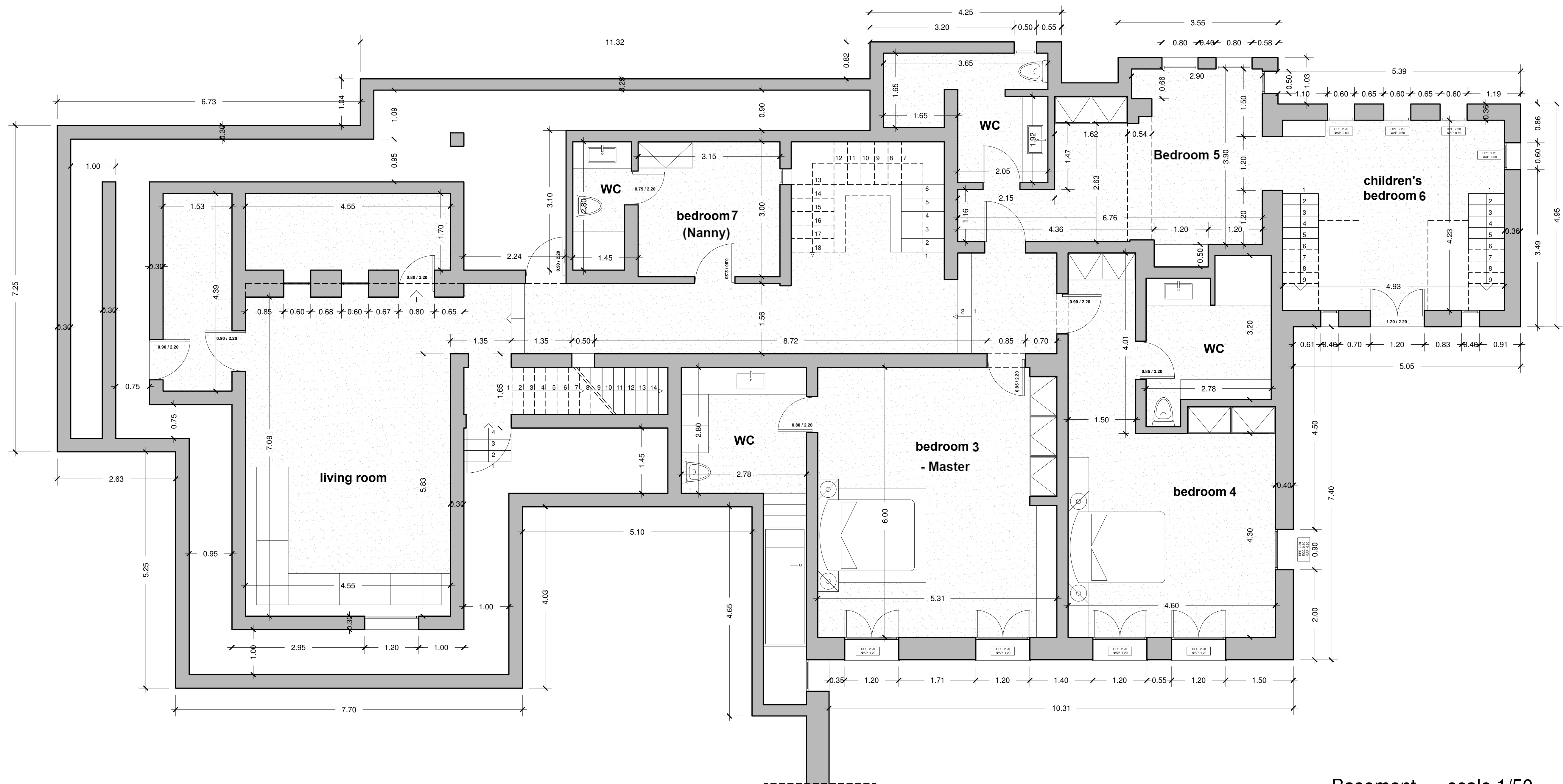
Basement__scale 1/50
