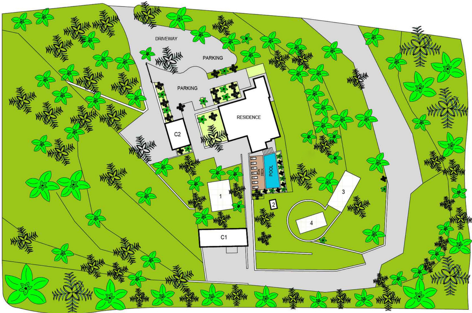
SITE PLAN
