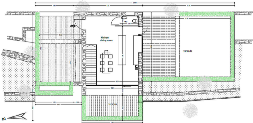
2nd level floor plan Area = 63,00m 2
