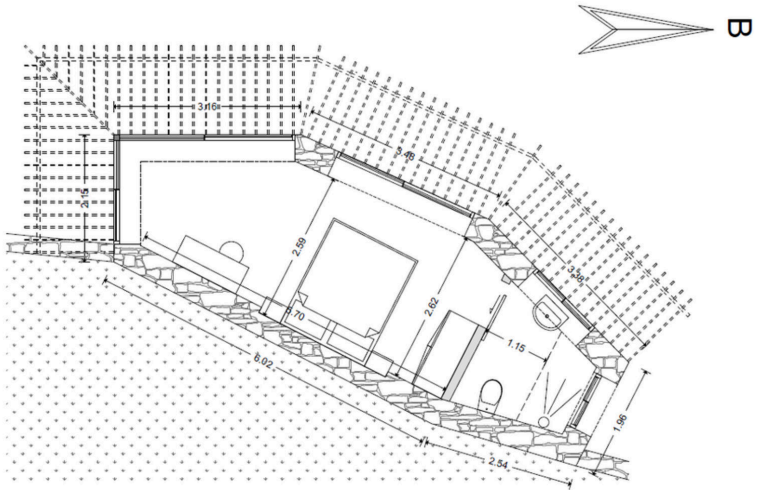
studio floor plan Area = 27,42m 2
