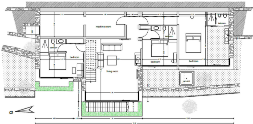
1st level floor plan Area = 207,79m 2
