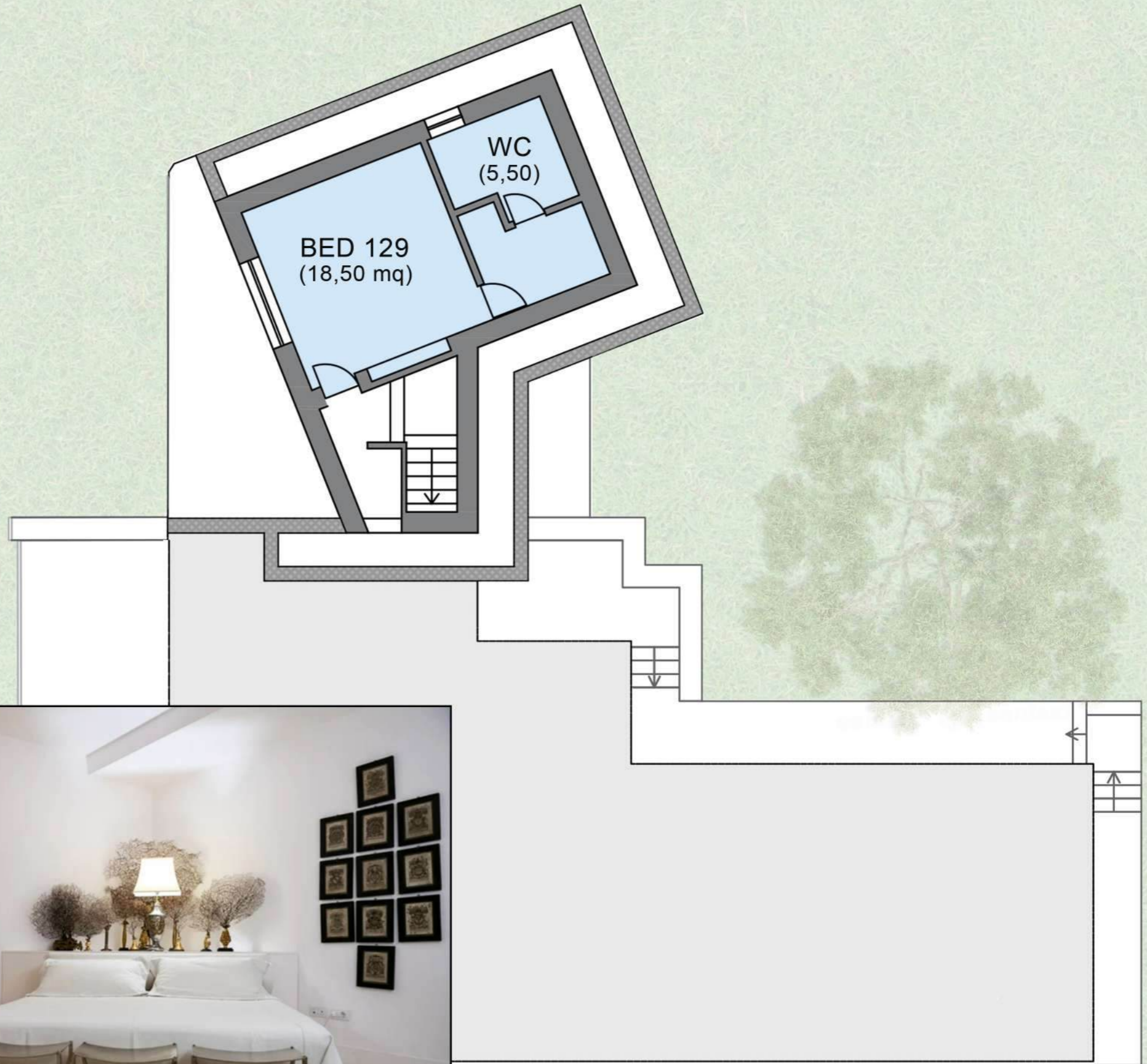
BASEMENT PLAN pianta piano interrato
