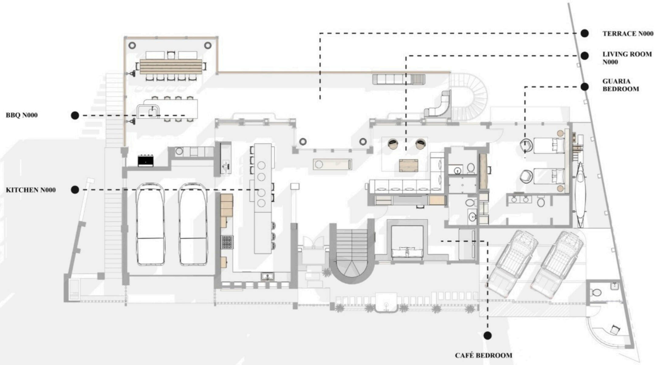
LEVEL TWO
