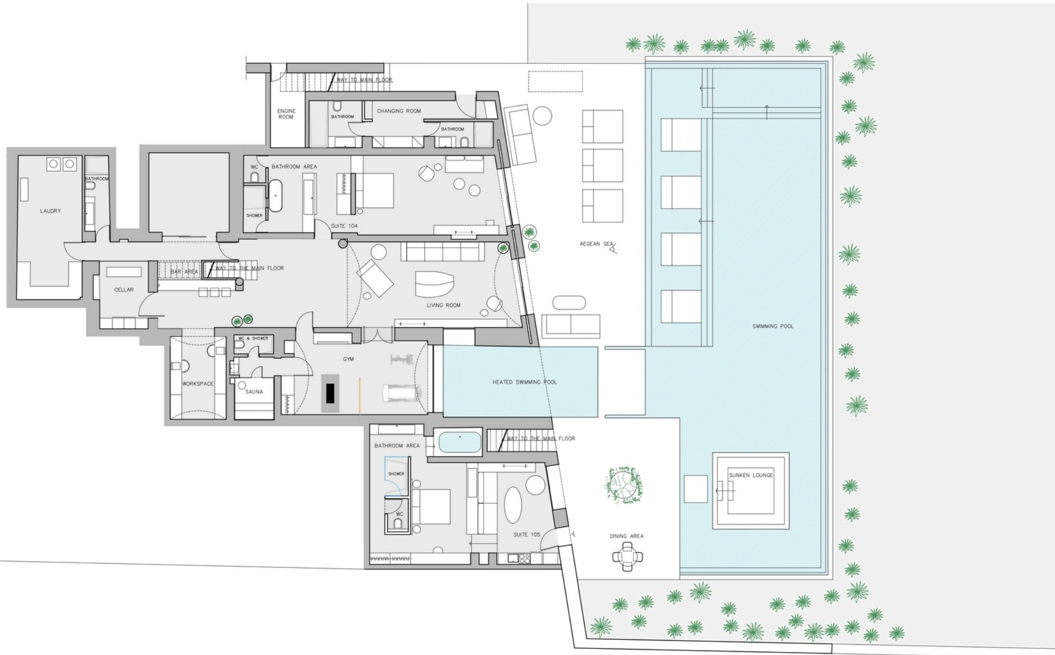
CHARISMA ESTATE FLOOR PLAN, POOL LEVEL
