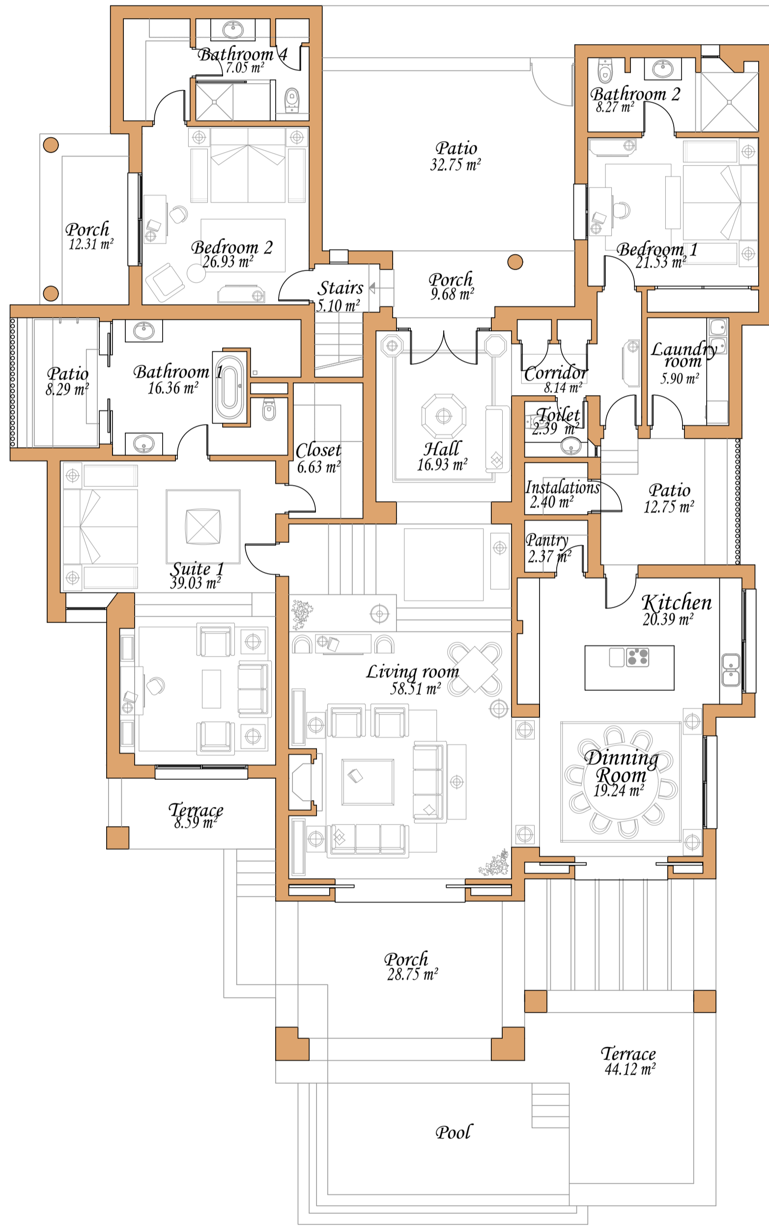
GROUND FLOOR
