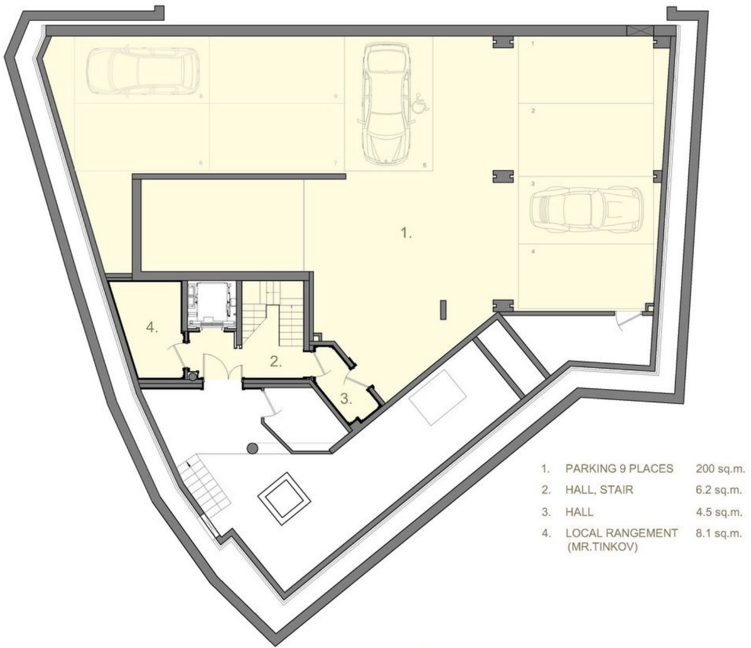
-3 level layout.
